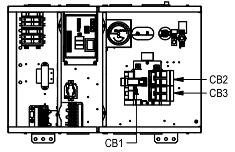
EH8 - EH20 1-PHASE SMALL BREAKER BASE
