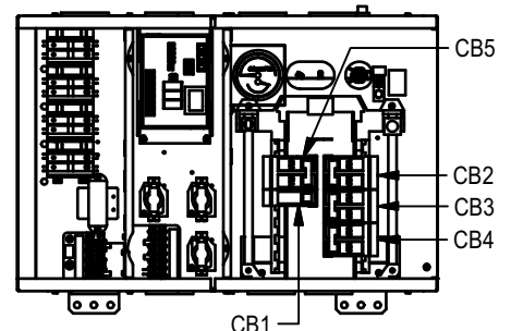
EH24 - EH40 1-PHASE LARGE BREAKER BASE
