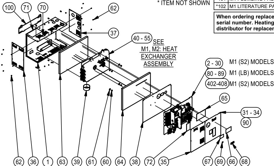
M1 (LB) WRAPPER WITH FUSE
