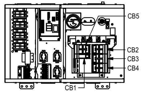
EH 32 - EH 40 3-PHASE BREAKER BASE
