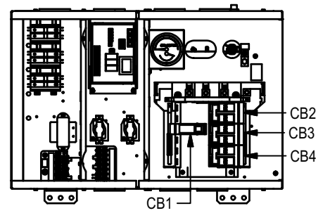
EH 12 - EH 30 3-PHASE BREAKER BASE
