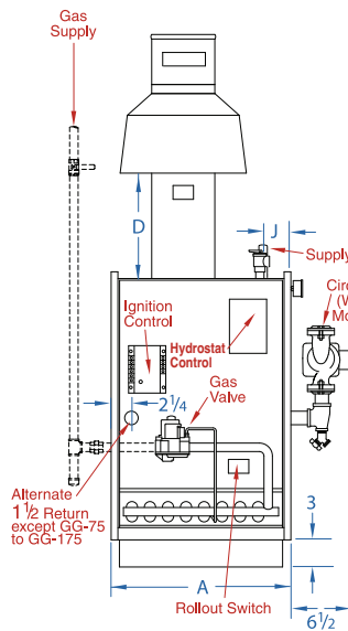
FRONT VIEW GG and GXHII Water Models
