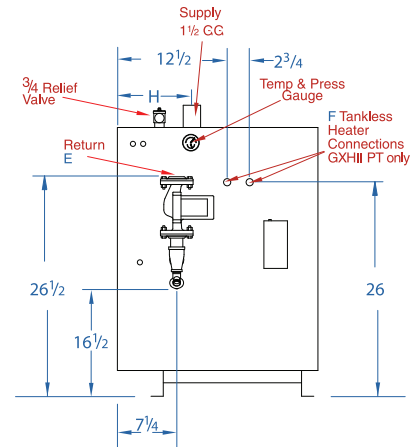
RIGHT SIDE VIEW GG and GXHII PT Water Models
