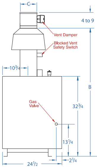
LEFT SIDE VIEW All GG and GXHII
